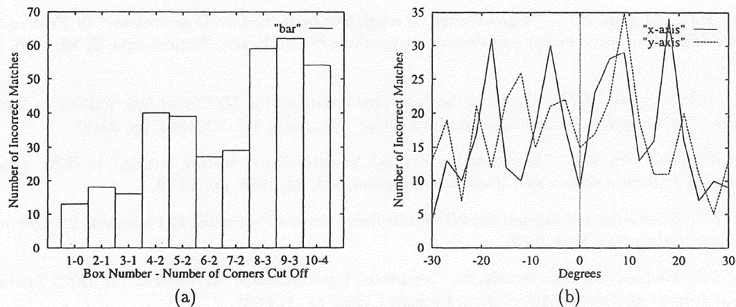
Figure 7: (a) Incorrect matches for each box (b) Incorrect matches for specific x and y-axis rotations (for all z-axis rotations).
