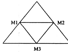
Figure 4: Multiresolution.
